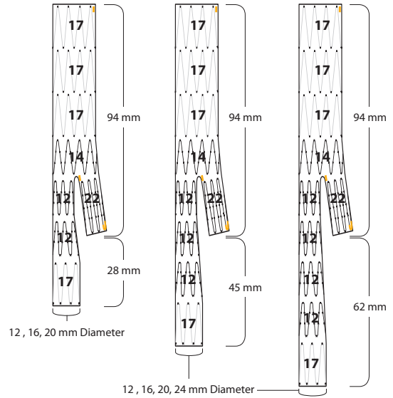
ZFEN-D-(12)(16)(20)(24)-(28)(45)(62)-94
